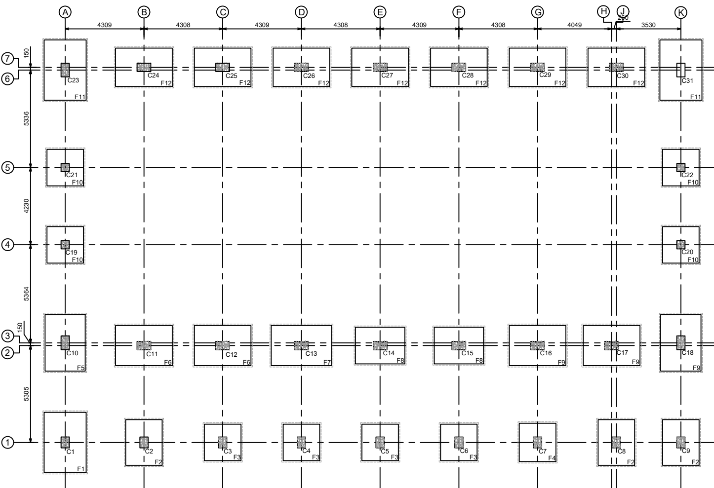
FOUNDATION PLAN SCALE- 1/25
